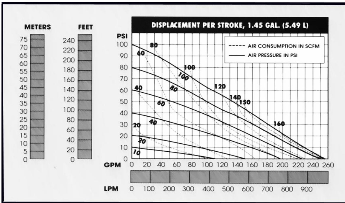
3" PERFORMANCE CURVE
